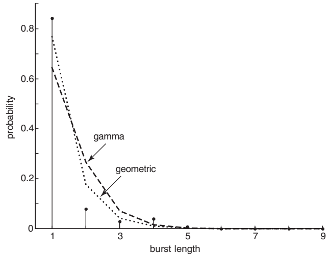
Fig. 3 Example of burst-length histogram (stems) in packet-loss bursts observed in SoLP
