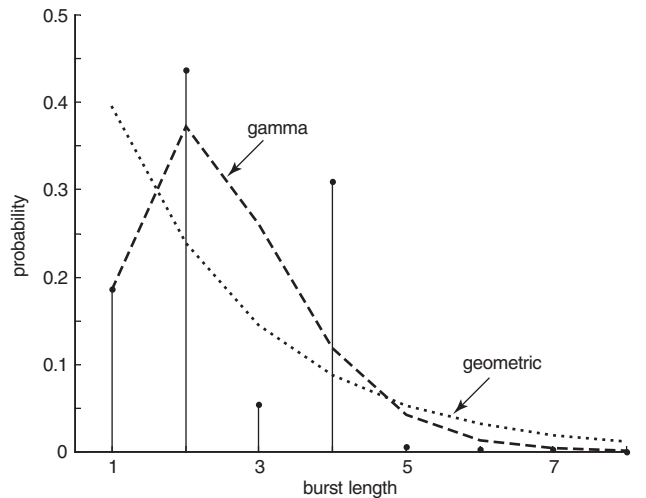
Fig. 4 Example of burst-length histogram (stems) in packet-loss bursts observed in SoLP
